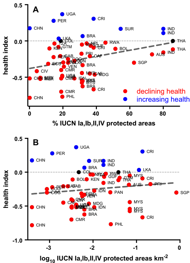
Fig. 2. Relationship between a protected area's health index and (A) the percentage of high-protection (IUCN categories Ia, b + II + IV) reserves by country in which the reserve is found ( R^2 = 0.11 ) and (B) the \log_{10} density of high-protection reserves per unit country area in which the reserve is found ( R^2 = 0.01 ). Indicative trend lines are fitted through the entire dataset in each case. Three-character ISO country codes are described at http://countrycode.org .
