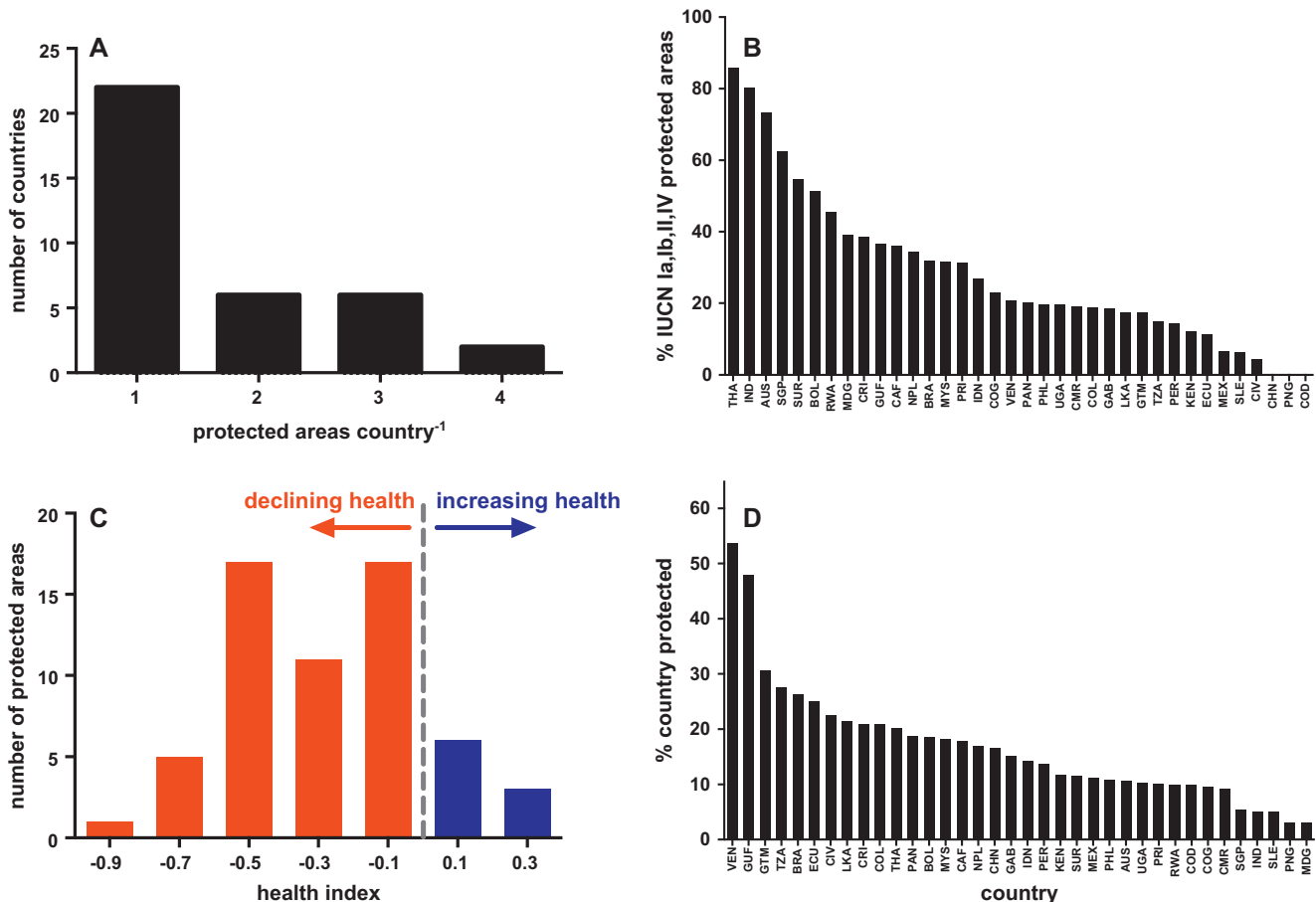
Fig. 1. Characteristics of protected areas in the sample of 60 reserves. (A) Number of protected areas per country (36 countries in total); (B) percentage of high-protection (IUCN categories Ia, b + II + IV) reserves by country; (C) distribution of the protected area 'health' index (Laurance et al., 2012); (D) percentage of the country under some form of protection by country. Three-character ISO country codes are described at http://countrycode.org .
